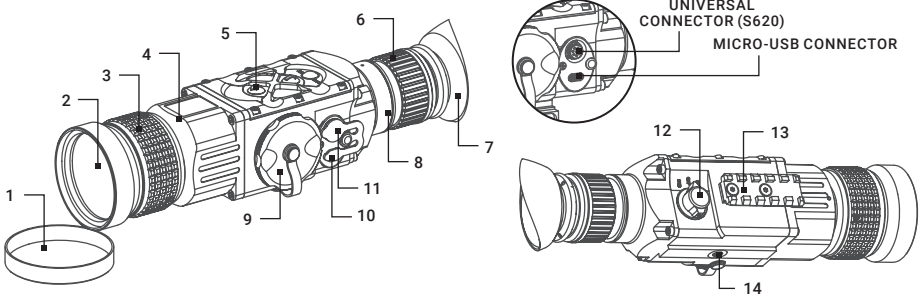
FIGURE 1-2. ASP THERMAL IMAGING MONOCULAR. SYSTEM DESCRIPTION
